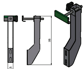
STAINLESS STEEL HOLDER + PLATE & WEAR STRIP
