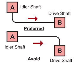
ARAH TRANSFER
