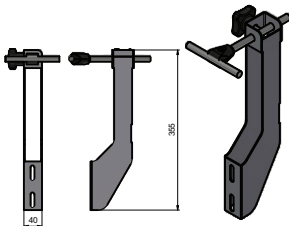
STAINLESS STEEL HOLDER + SINGLE ROUND BAR
