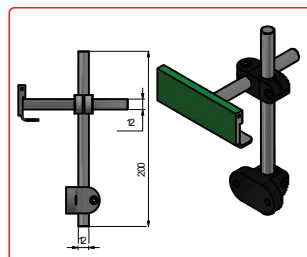
PLASTIC HOLDER CLAMP + PLATE & WEAR STRIP
