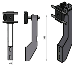
STAINLESS STEEL HOLDER + DOUBLE ROUND BAR
